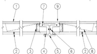
Figure 2.6. The picture shows an example of the connection between two adjacent HD elements in the lengthwise direction (Bygga med prefab 2008).
