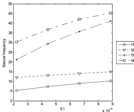
Figure 8.10. The figure shows how E1 influences the first four natural frequencies if everything else is kept constant.
