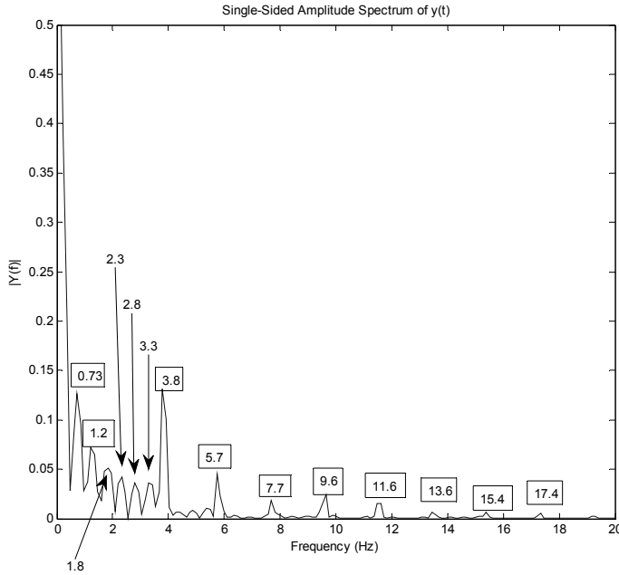
Figure 8.26. Frequency content of the load function f_{walk} = 1.9 Hz.
