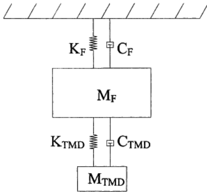
Figure 10.1. Model of a floor structure and a tuned mass damper. The parameters K_{TMD} , C_{TMD} and M_{TMD} must be carefully chosen (Ljunggren 2006).
