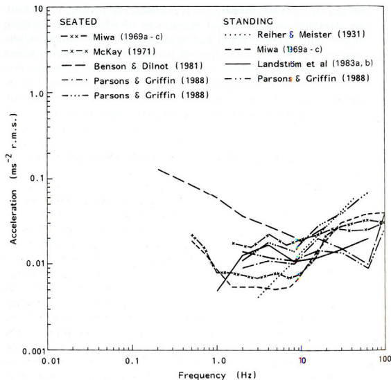
Figure 4.2. Perception thresholds for vertical whole-body vibration of seated and standing persons (Griffin 1990).
