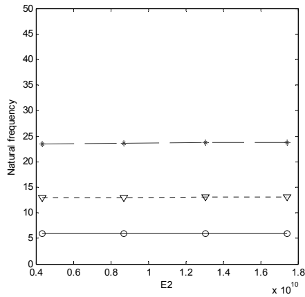
Figure 8.14. The figure shows how E2 influences the first three natural frequencies if everything else is kept constant.
