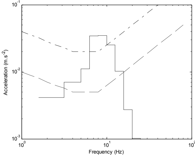
Figure 8.32. Acceleration magnitudes in 1/3 octave bands at the midpoint of the floor, without a concrete topping. Span of the floor: 7m. The diagram also shows the base curve of ISO 2631-2:1989, and the curve that is valid for offices.
