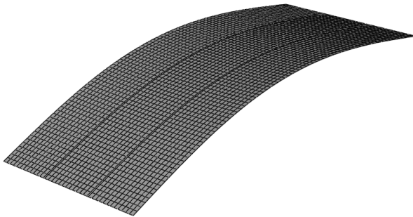
Figure 8.7. Mode shape 1.
