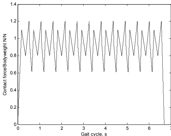
Figure 8.23. Reaction force time history for 12 footsteps. f_{walk} = 1.8 Hz.
