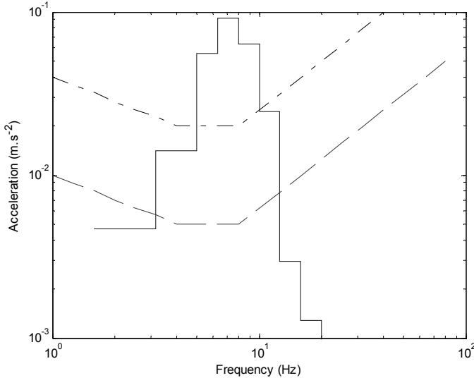
Figure 8.28. Acceleration magnitudes in 1/3 octave bands at the location rms10, without a concrete topping. The diagram also shows the base curve of ISO 2631-2:1989, and the curve that is valid for offices.
