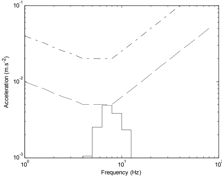
Figure 7.12. Acceleration magnitudes in 1/3 octave bands ( t=10s ) at the location of the chair, caused by the same walker as in the subjective tests. The diagram also shows the base curve of ISO 2631-2:1989, and the curve that is valid for offices.
