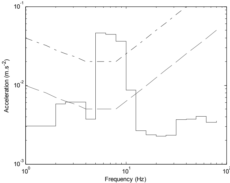
Figure 7.13. Acceleration magnitudes in 1/3 octave bands at the location of the chair, caused by the same walker as in the subjective tests. The diagram also shows the base curve of ISO 2631-2:1989, and the curve that is valid for offices.
