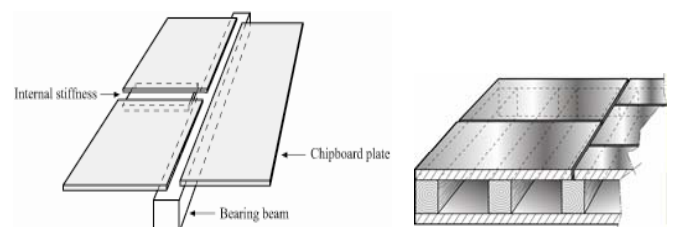
Figure 1.-Floor structure,
